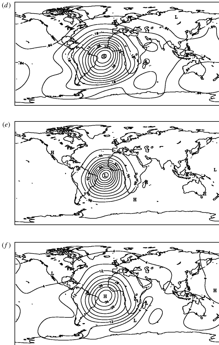
Figure 1. ( Cont. ) ( d ) The average directional variation \partial_t A ( \text{deg yr}^{-1} ), equation (4.5); global average: 4.4^\circ per century. ( e ) The angular correlation r between vectors at 1840 and 1990, equation (4.6); global average: 0.9956. ( f ) The angular difference \xi between vectors at 1840 and 1990, equation (4.7); global average 5.4^\circ . Note that the total secular variation \partial_t B is highest in the middle of the Atlantic, where the intensity is lowest. Most of this correlation is due to the angular secular variation \partial_t A ; the correlation of relative intensity variation \partial_t F with the intensity low is not as good. L denotes low, H denotes high.
