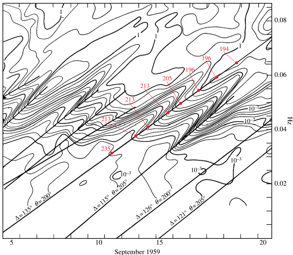
Figure 1. Contours of power density E(t, f) in units \text{m}^2 \text{Hz}^{-1} (ticks on the t -axis designate midnight Universal Time) recorded at San Clemente Island. Ridge lines f = m(t - t_0) correspond to the dispersive arrivals from a single source at time t_0 and range g/(4\pi m) . For the 4.5 September 1959 event (centred midday 4 September), the range is 15 390 km; measured azimuths ( \alpha = 180^\circ from south and 270^\circ from west) at the points along the ridge line vary from \alpha = 213^\circ on 12 September ( f = 0.037 Hz) to \alpha = 196^\circ on 17 September ( f = 0.06 Hz). (Online version in colour.)
