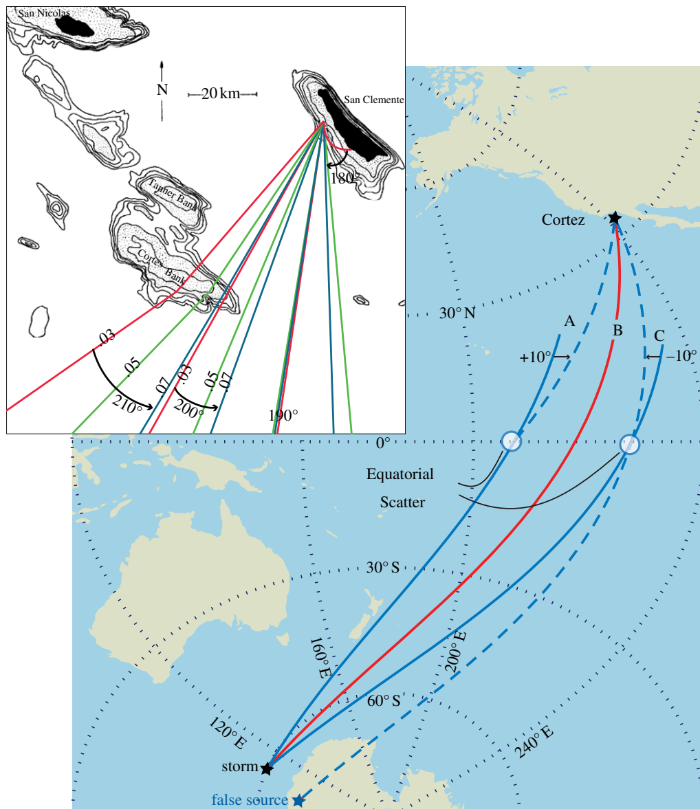
Figure 2. Wave trajectories from the Indian Ocean to California. Early low-frequency arrivals clearly follow a great circle trajectory (line B) leaving the storm in indirection \theta = \alpha - 180^\circ = 107^\circ ( \theta = 0^\circ towards north and 90^\circ towards east), crossing the equator at \theta = 29^\circ and arriving at Cortez Bank at \theta = 35^\circ , \alpha = 215^\circ (table 1); further progress is impeded (Inset by O'Reilly shows bathymetric refraction, depth contours 0, 50, 150, 200, 250 fm). Later high-frequency arrivals are scattered at the equator by \pm 10^\circ (dashed line A, C). Rays A and B are partially blocked by Cortez Bank, C reaches the San Clemente wave array with \theta = 19^\circ , \alpha = 199^\circ . Neglect of equatorial scatter places the wave-inferred source on Antarctica (dashed). (Online version in colour.)
