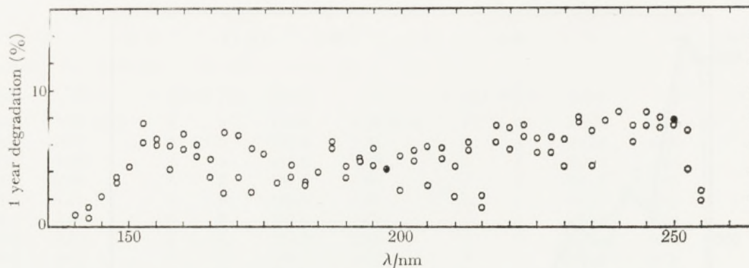
FIGURE 5. Average decrease of sensitivity for channels 2, 3 and 4 over a period of 1 year.
